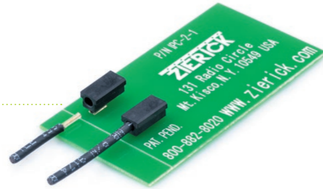
Surface mount coax cable connector
