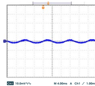
Output Ripple & Noise
