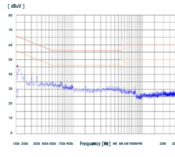
Daitron switching power supply
